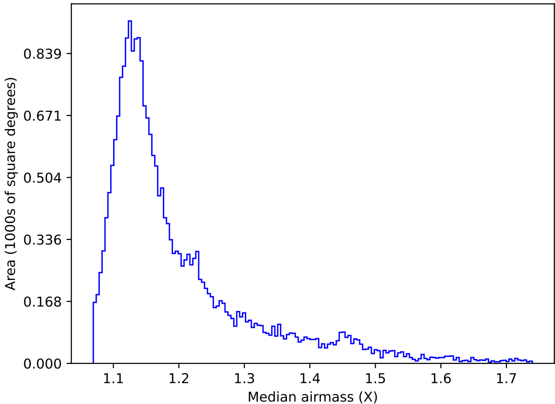
too_elab_r16_d3_gz_v3.4_10yrs All sky u band: Median airmass
