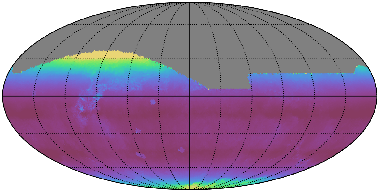
too_elab_r16_d3_gz_v3.4_10yrs All sky r band: Median airmass
