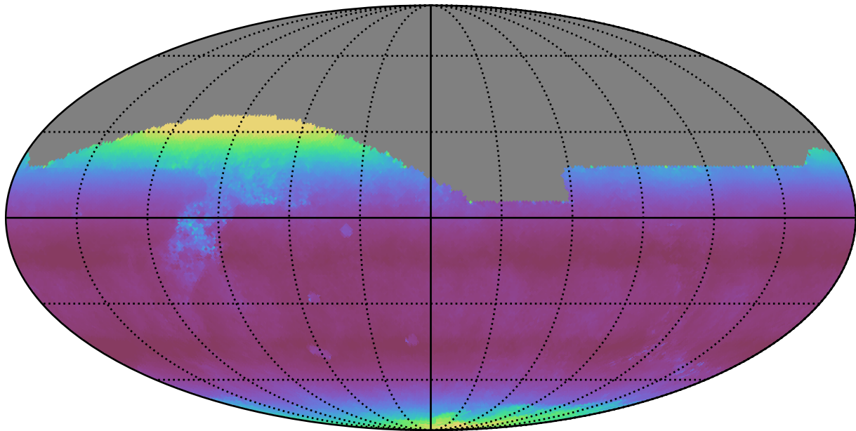
too_elab_r16_d3_gz_v3.4_10yrs All sky i band: Median airmass
