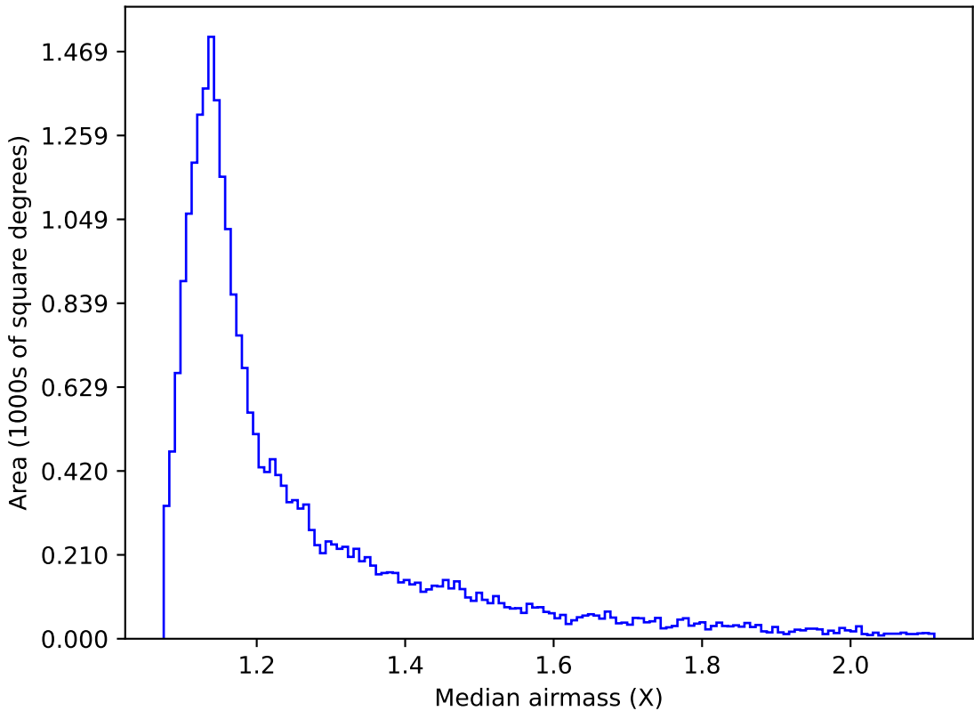
too_elab_r16_d3_gz_v3.4_10yrs All sky g band: Median airmass
