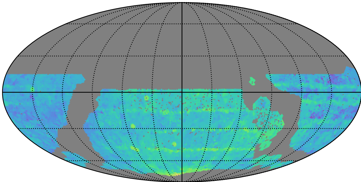
too_elab_r16_d3_gz_v3.4_10yrs WFD z band: Median Season Length
