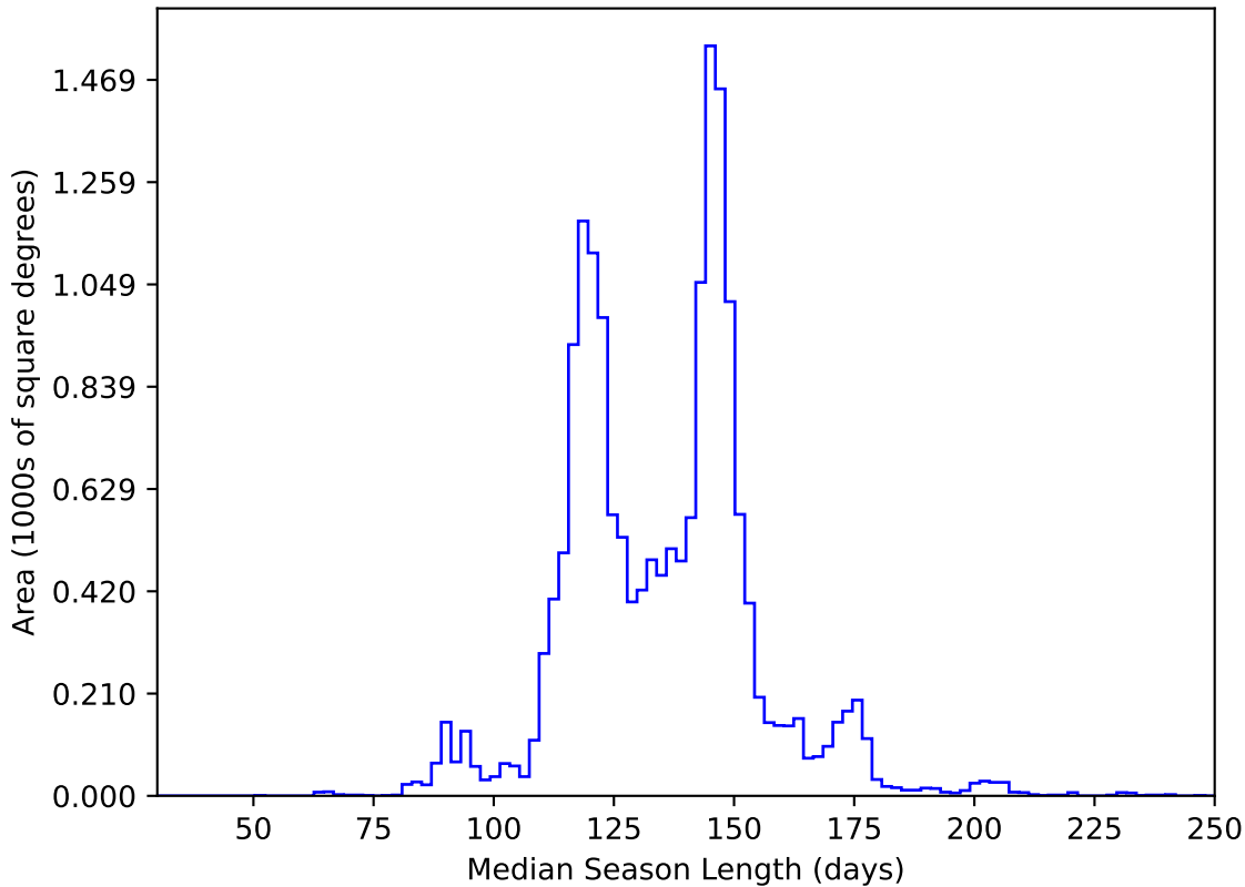
too_elab_r16_d3_gz_v3.4_10yrs WFD y band: Median Season Length
