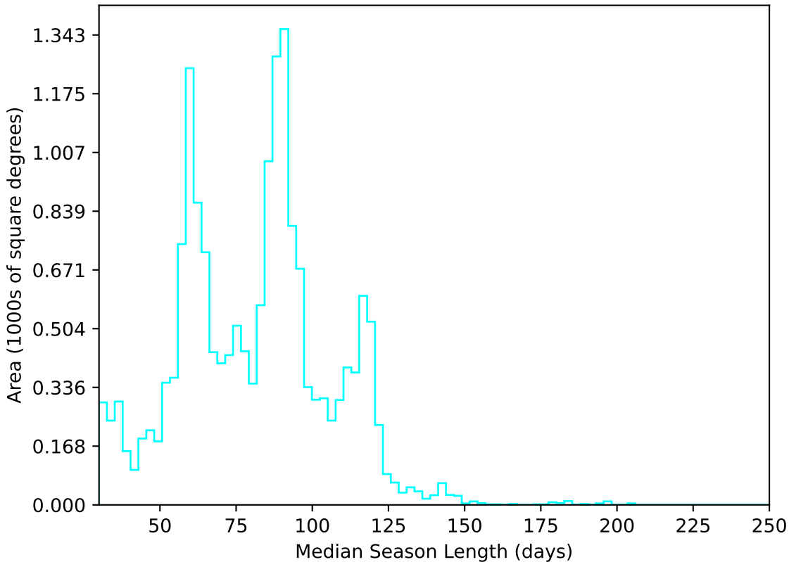
too_elab_r16_d3_gz_v3.4_10yrs WFD u band: Median Season Length
