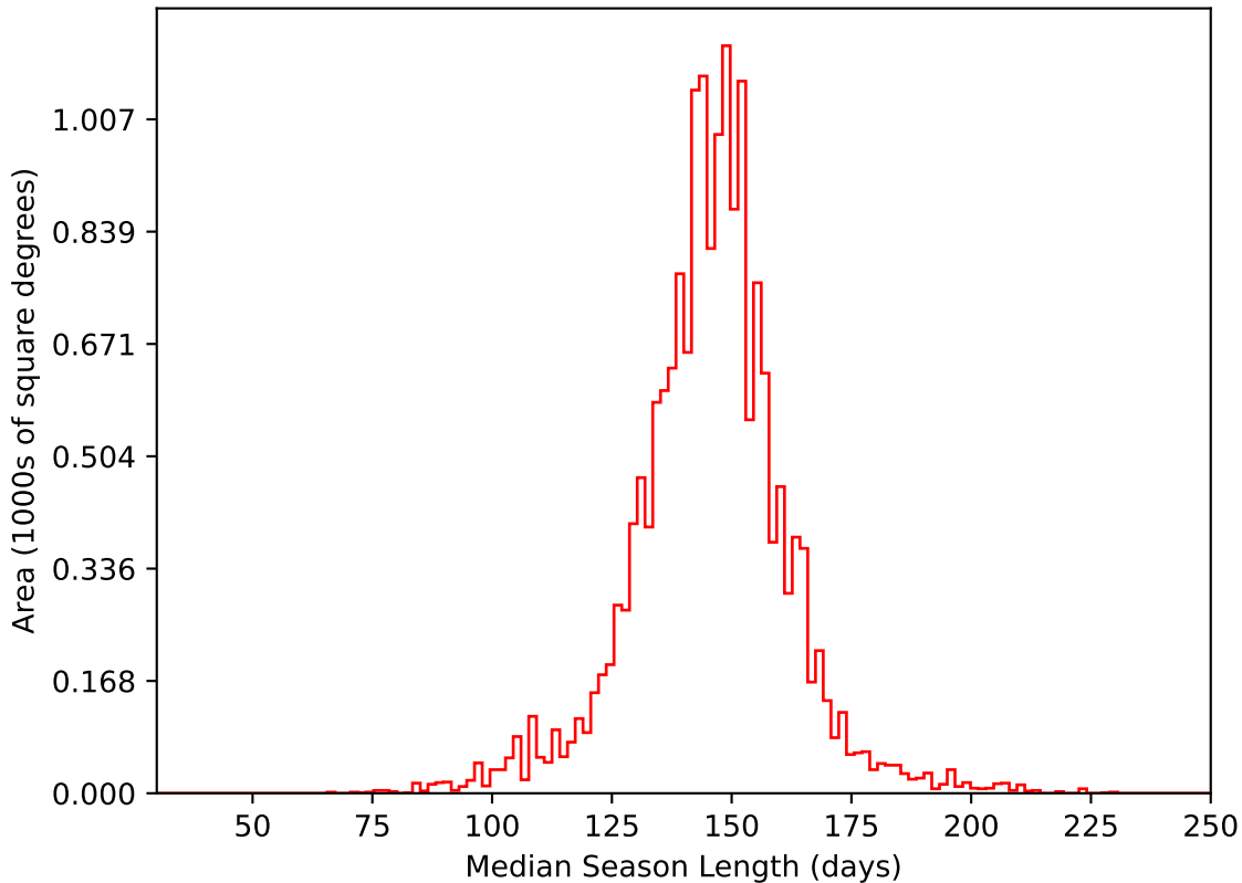
too_elab_r16_d3_gz_v3.4_10yrs WFD i band: Median Season Length
