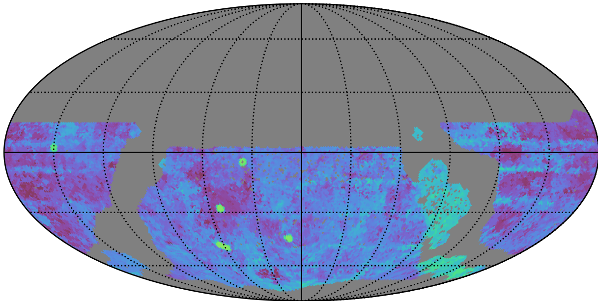
too_elab_r16_d3_gz_v3.4_10yrs WFD g band: Median Season Length
