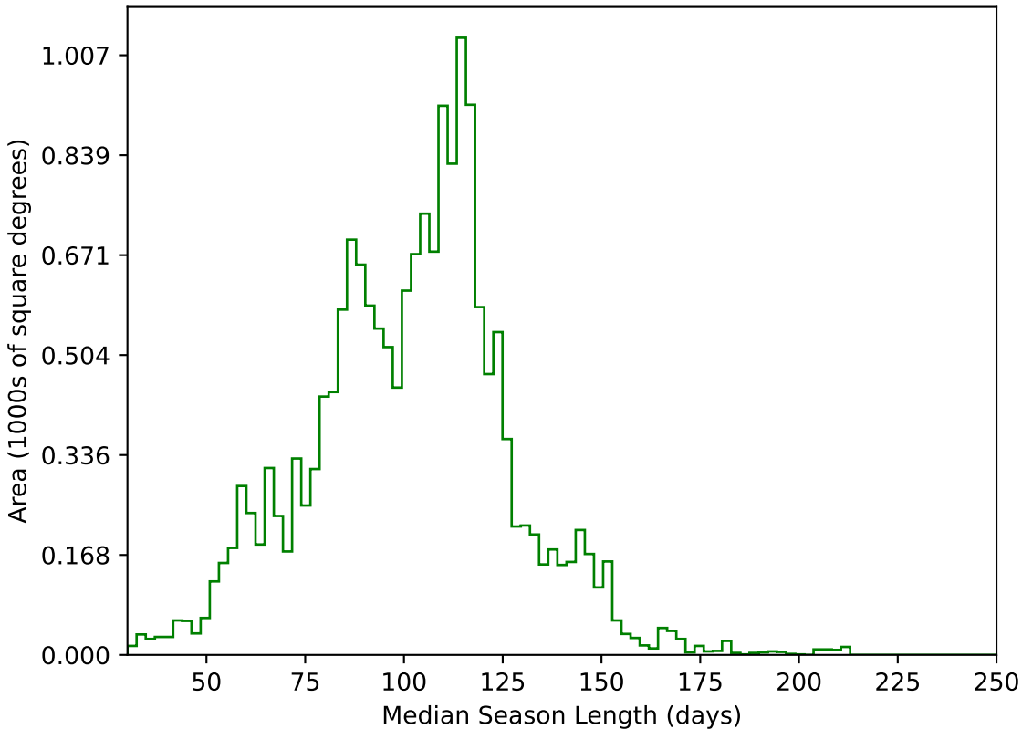
too_elab_r16_d3_gz_v3.4_10yrs WFD g band: Median Season Length
