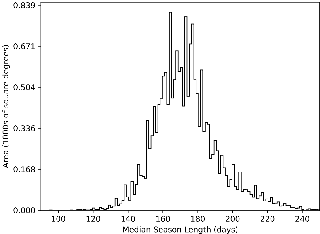
too_elab_r16_d3_gz_v3.4_10yrs WFD all bands: Median Season Length
