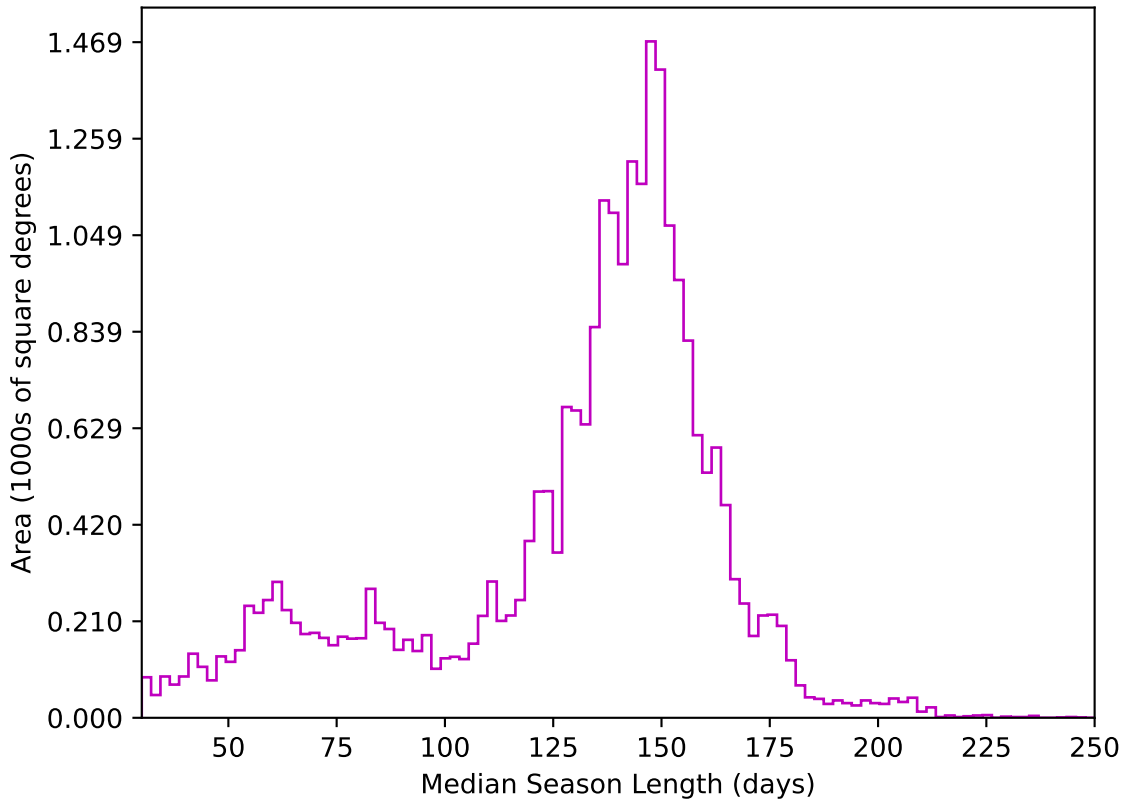
too_elab_r16_d3_gz_v3.4_10yrs All sky z band: Median Season Length
