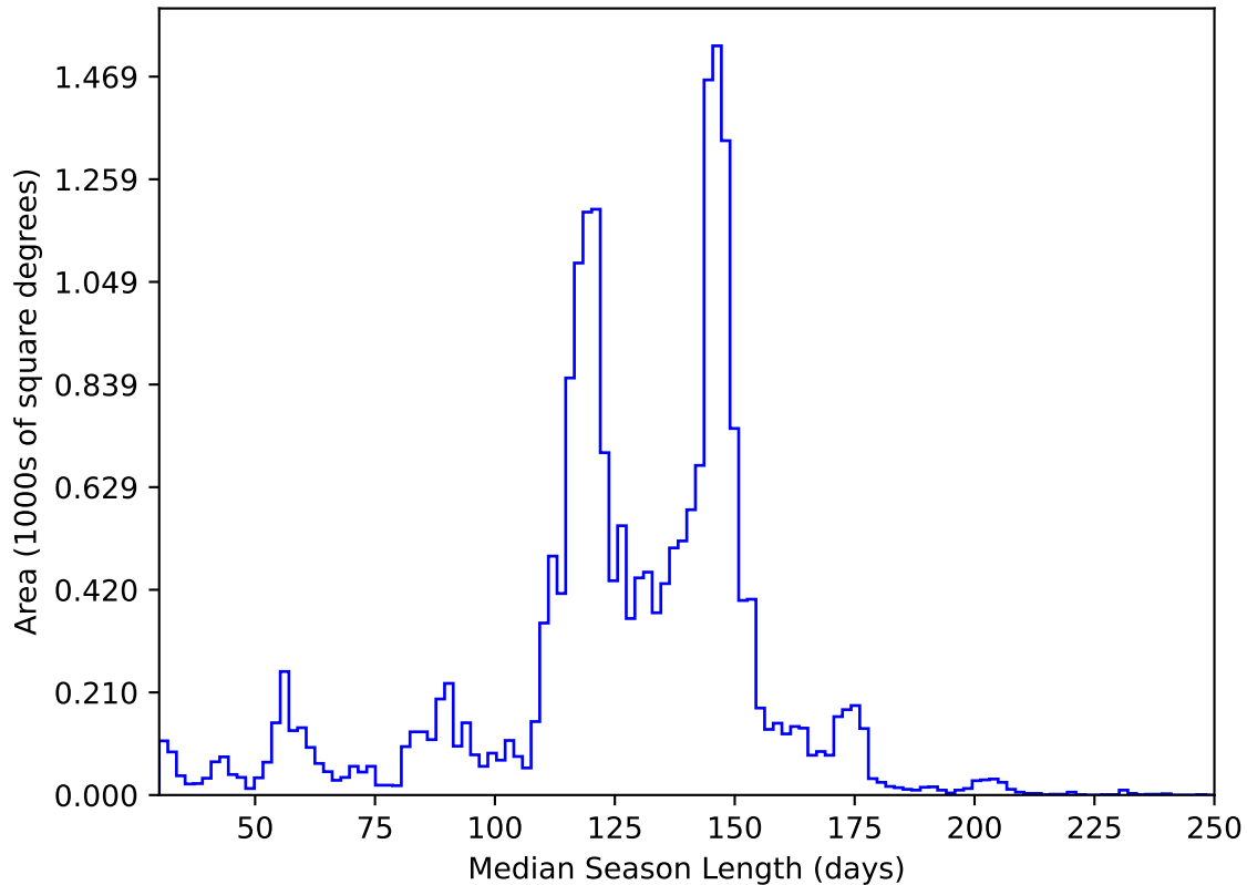
too_elab_r16_d3_gz_v3.4_10yrs All sky y band: Median Season Length
