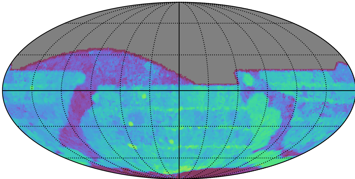
too_elab_r16_d3_gz_v3.4_10yrs All sky r band: Median Season Length
