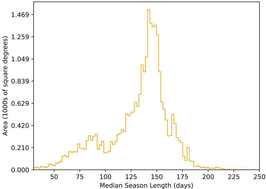
too_elab_r16_d3_gz_v3.4_10yrs All sky r band: Median Season Length
