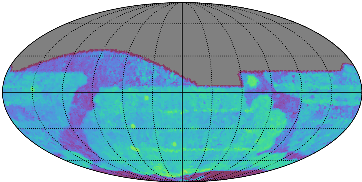
too_elab_r16_d3_gz_v3.4_10yrs All sky i band: Median Season Length
