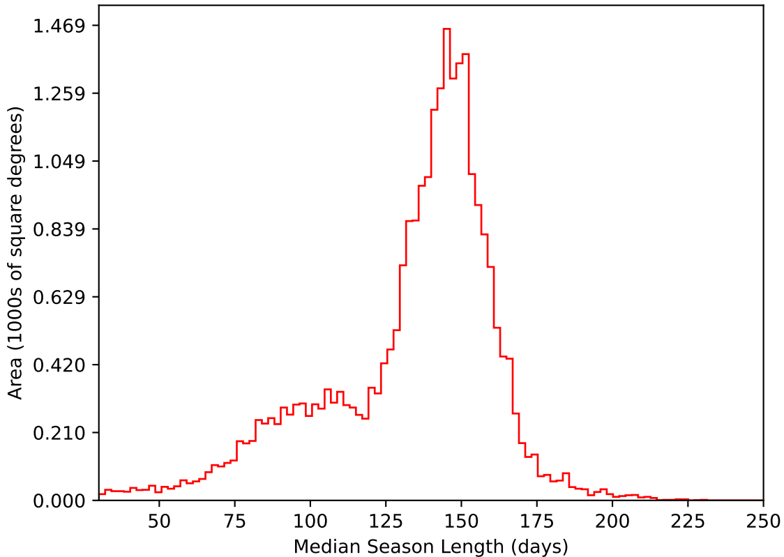
too_elab_r16_d3_gz_v3.4_10yrs All sky i band: Median Season Length
