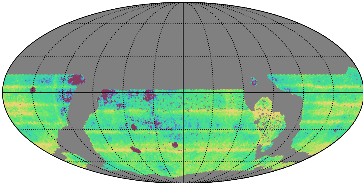
too_elab_r16_d3_gz_v3.4_10yrs WFD: Median Intra-Night Gap
