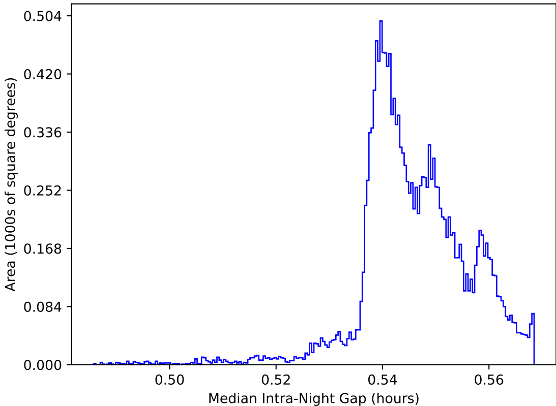
too_elab_r16_d3_gz_v3.4_10yrs WFD: Median Intra-Night Gap
