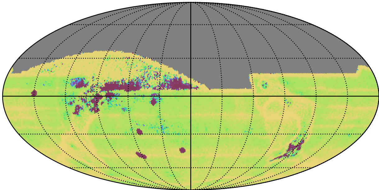
too_elab_r16_d3_gz_v3.4_10yrs All sky: Median Intra-Night Gap
