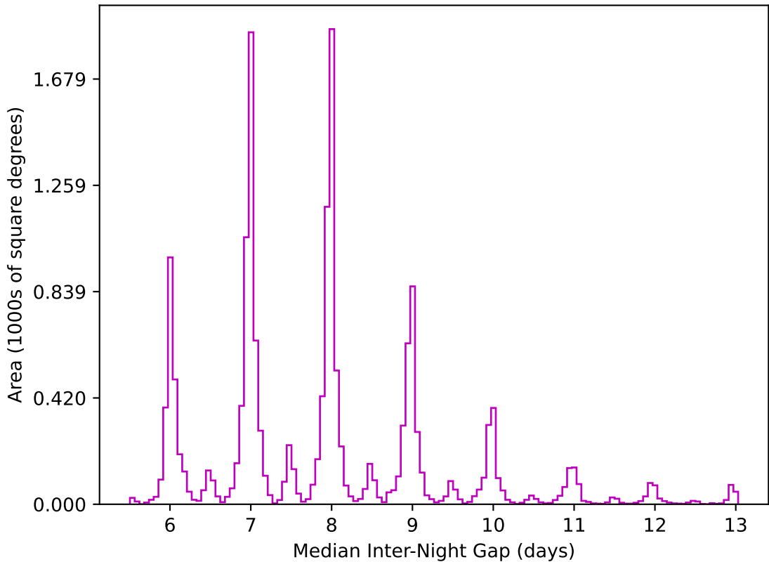
too_elab_r16_d3_gz_v3.4_10yrs WFD z band: Median Inter-Night Gap
