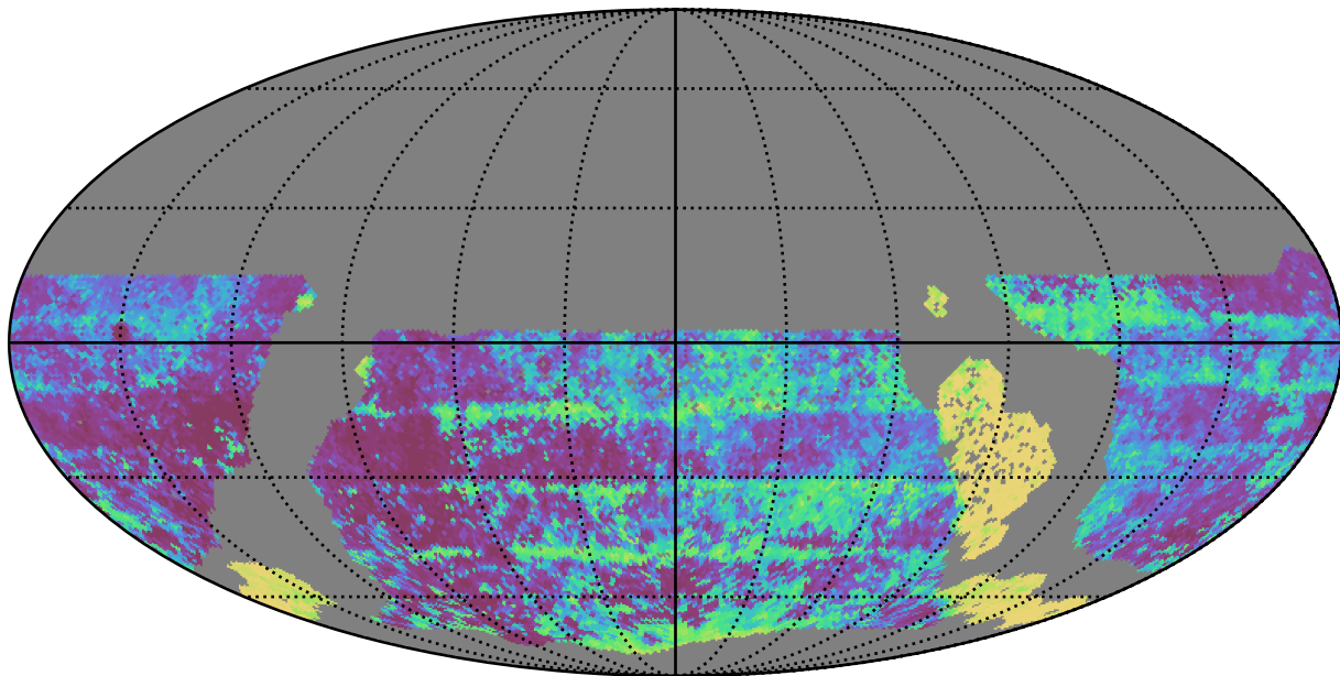
too_elab_r16_d3_gz_v3.4_10yrs WFD y band: Median Inter-Night Gap
