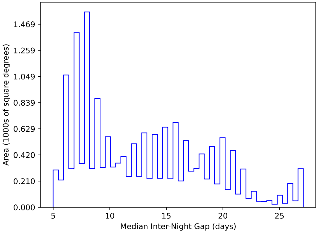
too_elab_r16_d3_gz_v3.4_10yrs WFD y band: Median Inter-Night Gap
