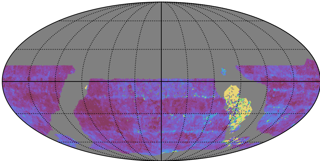
too_elab_r16_d3_gz_v3.4_10yrs WFD u band: Median Inter-Night Gap
