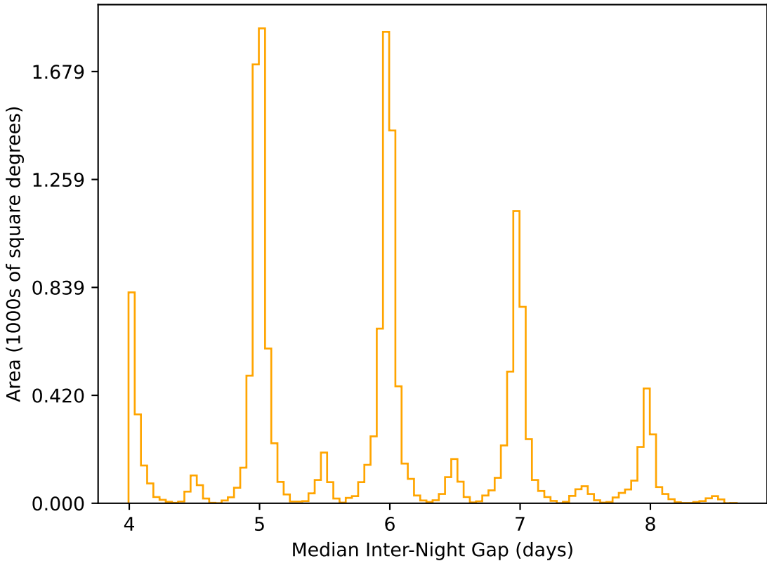
too_elab_r16_d3_gz_v3.4_10yrs WFD r band: Median Inter-Night Gap
