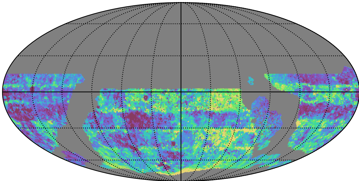
too_elab_r16_d3_gz_v3.4_10yrs WFD g band: Median Inter-Night Gap
