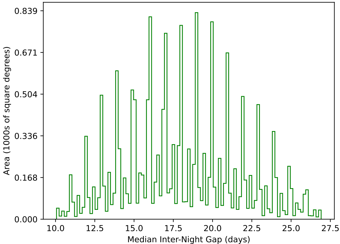
too_elab_r16_d3_gz_v3.4_10yrs WFD g band: Median Inter-Night Gap
