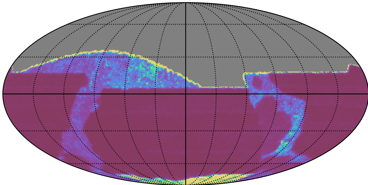
too_elab_r16_d3_gz_v3.4_10yrs All sky z band: Median Inter-Night Gap
