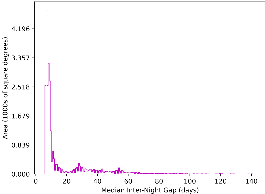
too_elab_r16_d3_gz_v3.4_10yrs All sky z band: Median Inter-Night Gap
