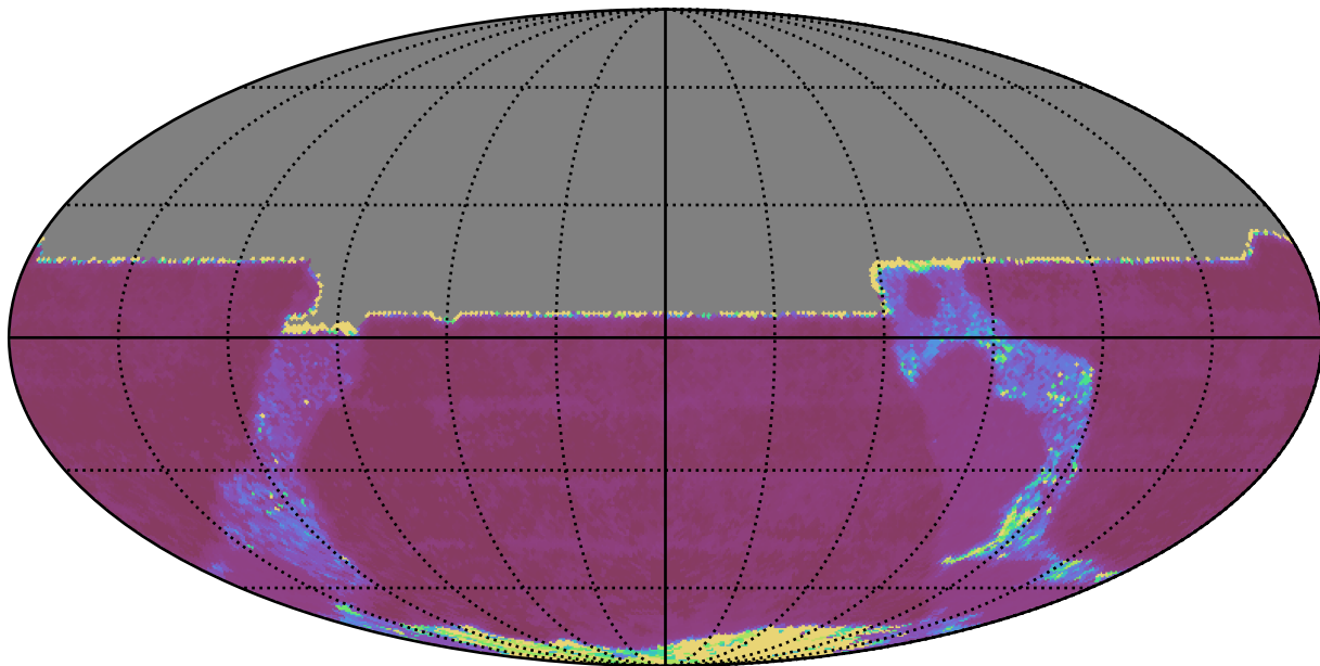
too_elab_r16_d3_gz_v3.4_10yrs All sky y band: Median Inter-Night Gap
