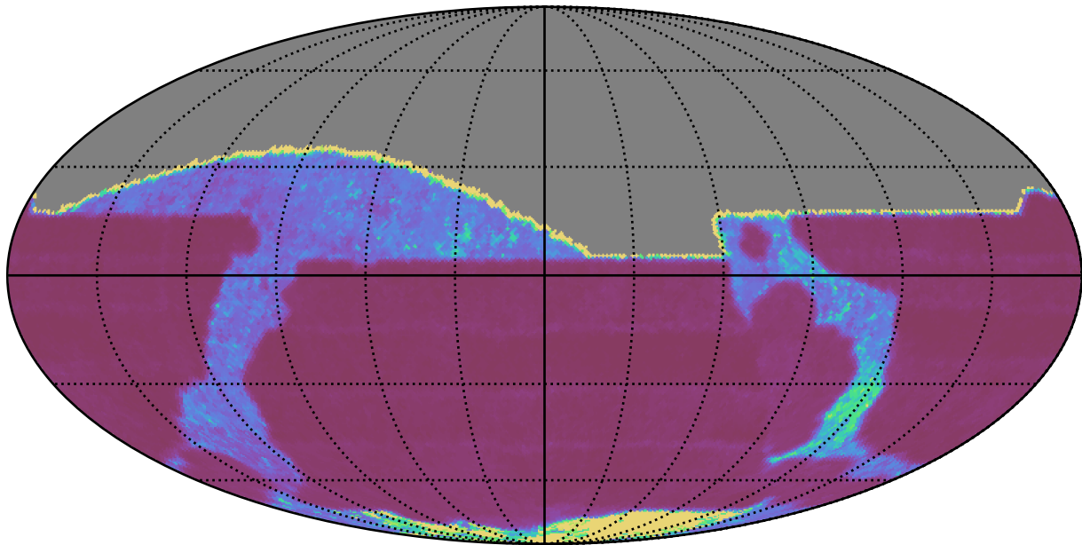
too_elab_r16_d3_gz_v3.4_10yrs All sky r band: Median Inter-Night Gap
