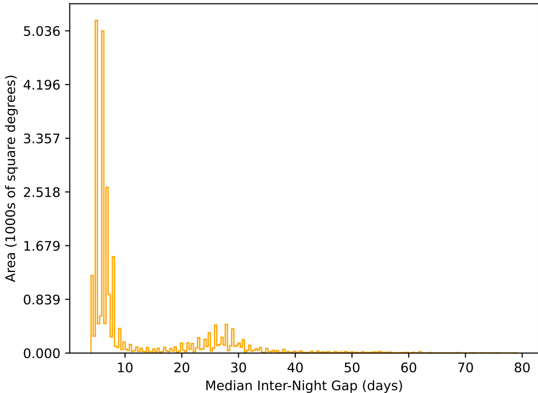
too_elab_r16_d3_gz_v3.4_10yrs All sky r band: Median Inter-Night Gap
