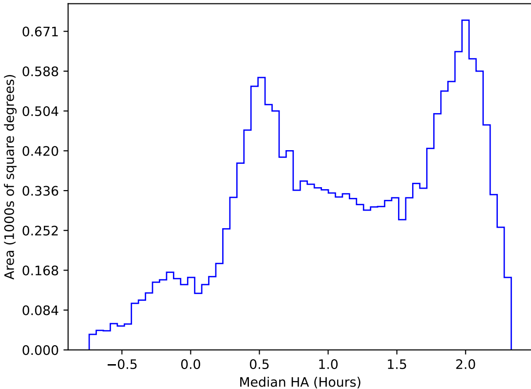
too_elab_r16_d3_gz_v3.4_10yrs WFD z band: Median HA
