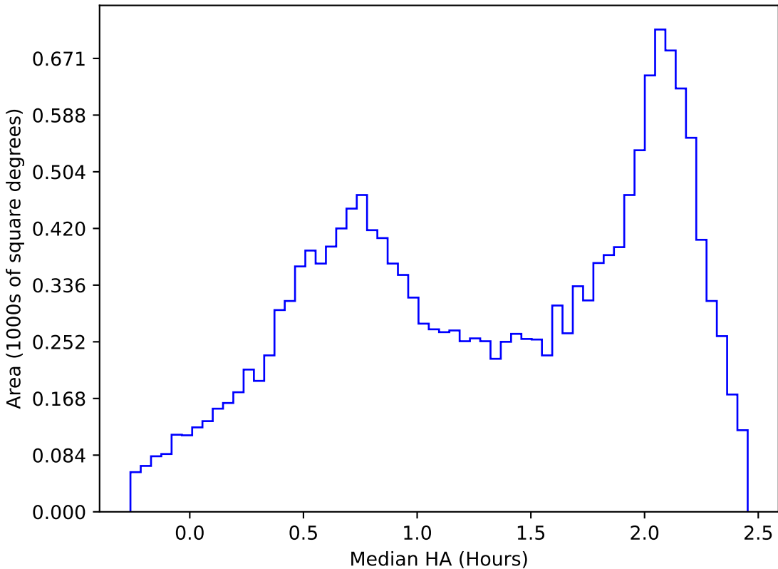
too_elab_r16_d3_gz_v3.4_10yrs WFD y band: Median HA
