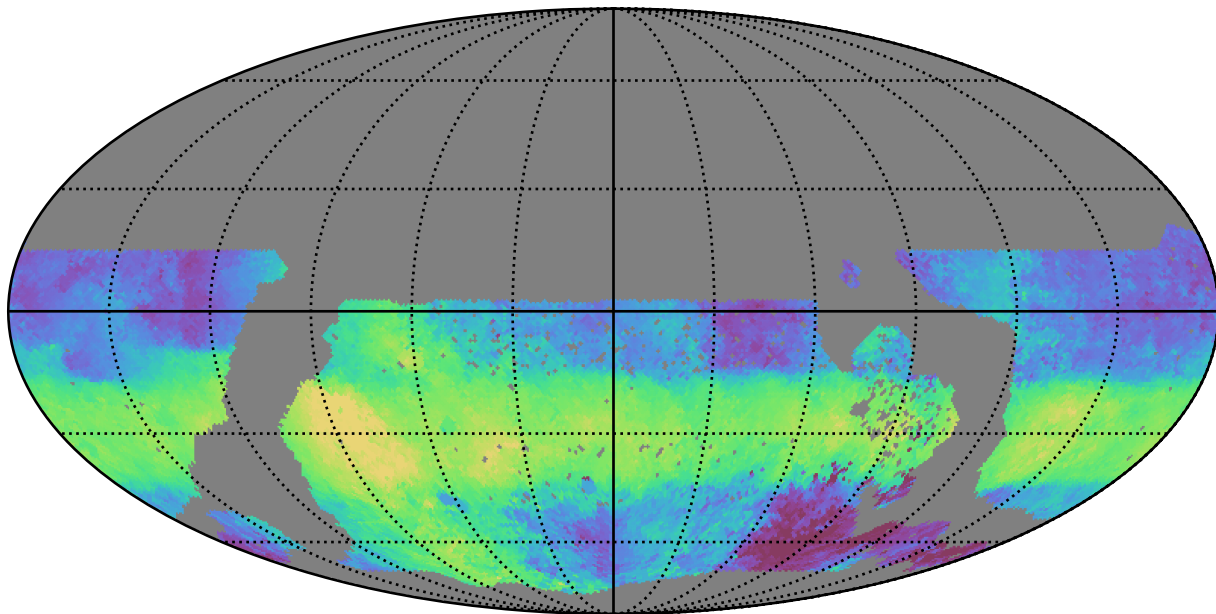
too_elab_r16_d3_gz_v3.4_10yrs WFD u band: Median HA
