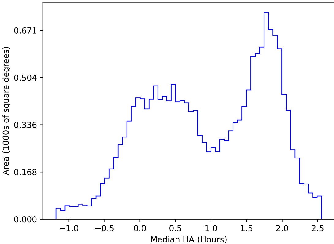
too_elab_r16_d3_gz_v3.4_10yrs WFD u band: Median HA
