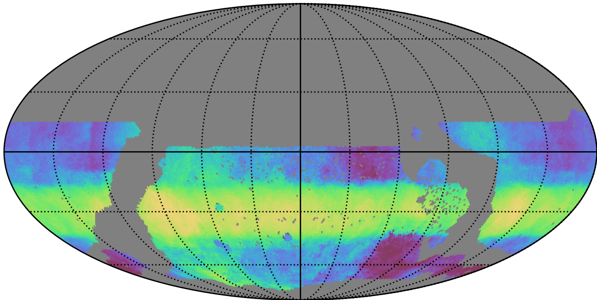
too_elab_r16_d3_gz_v3.4_10yrs WFD r band: Median HA
