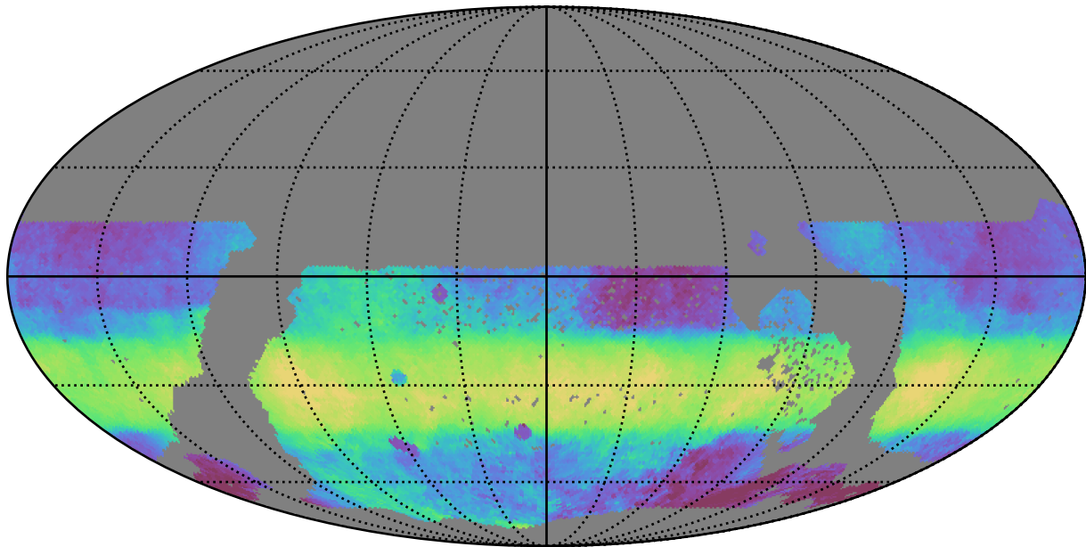
too_elab_r16_d3_gz_v3.4_10yrs WFD i band: Median HA
