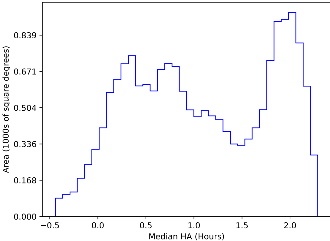
too_elab_r16_d3_gz_v3.4_10yrs WFD i band: Median HA
