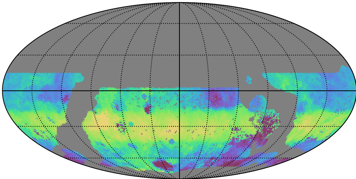
too_elab_r16_d3_gz_v3.4_10yrs WFD g band: Median HA
