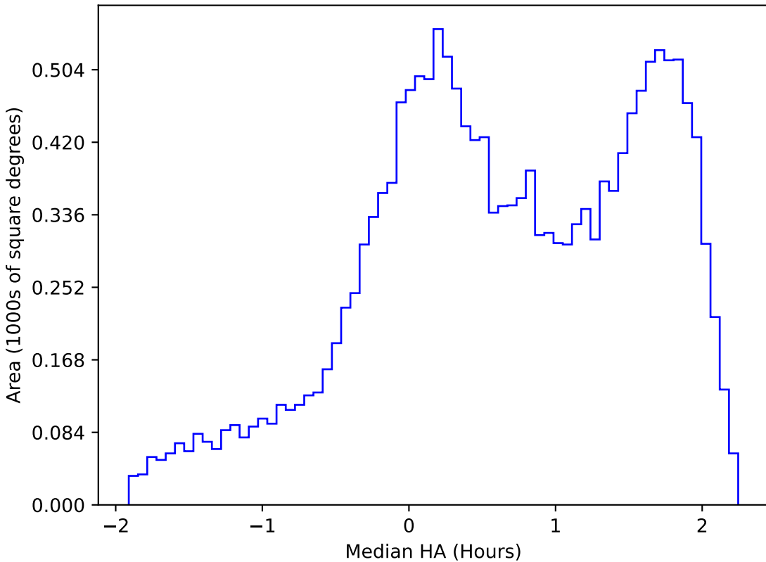
too_elab_r16_d3_gz_v3.4_10yrs WFD g band: Median HA
