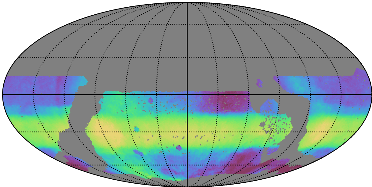
too_elab_r16_d3_gz_v3.4_10yrs WFD all bands: Median HA
