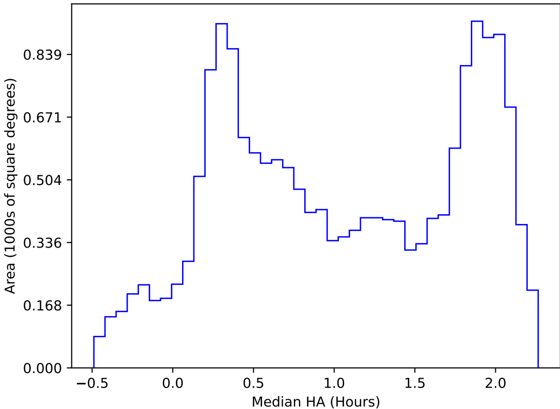
too_elab_r16_d3_gz_v3.4_10yrs WFD all bands: Median HA
