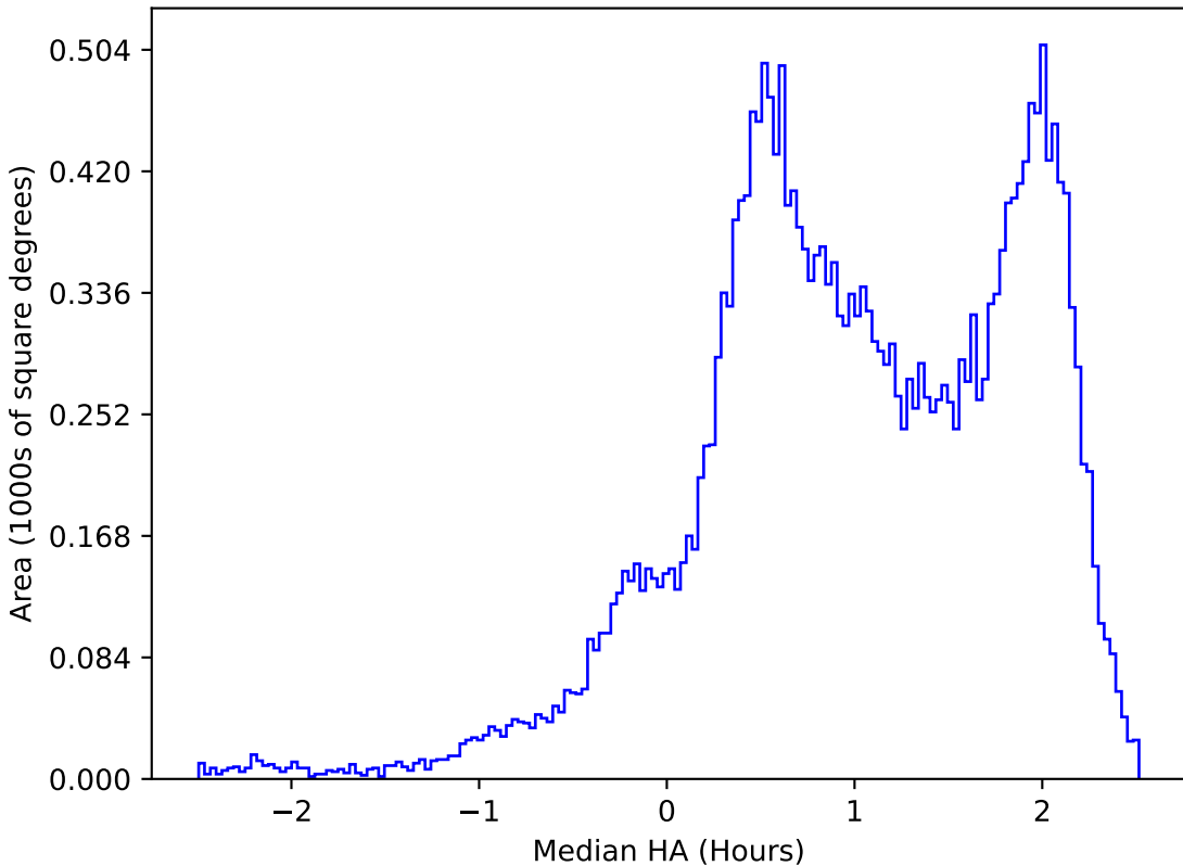
too_elab_r16_d3_gz_v3.4_10yrs All sky z band: Median HA
