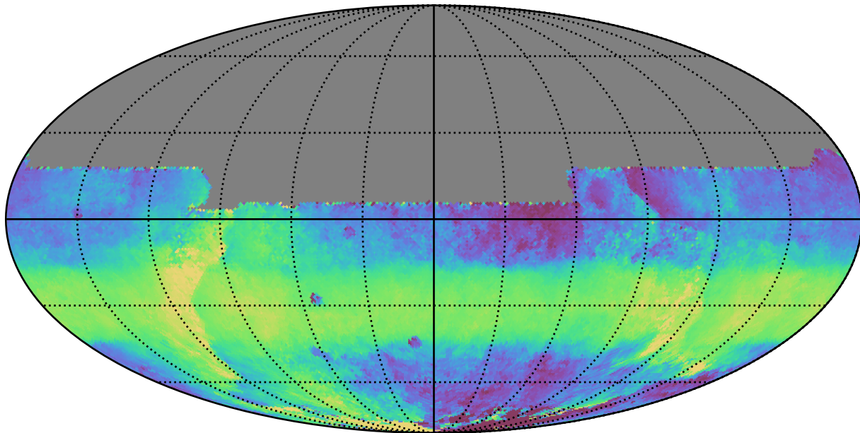
too_elab_r16_d3_gz_v3.4_10yrs All sky y band: Median HA
