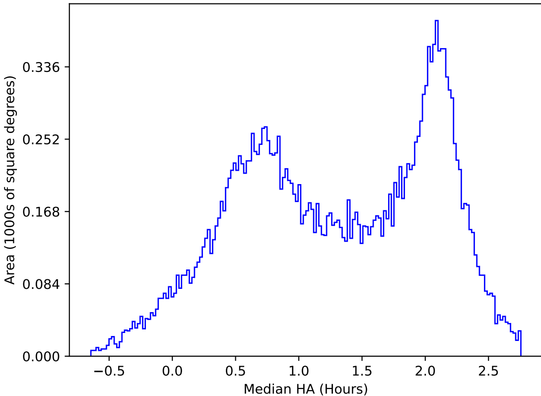
too_elab_r16_d3_gz_v3.4_10yrs All sky y band: Median HA
