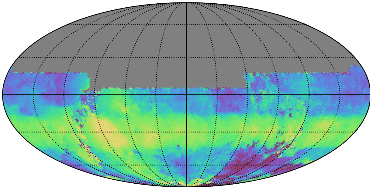
too_elab_r16_d3_gz_v3.4_10yrs All sky u band: Median HA
