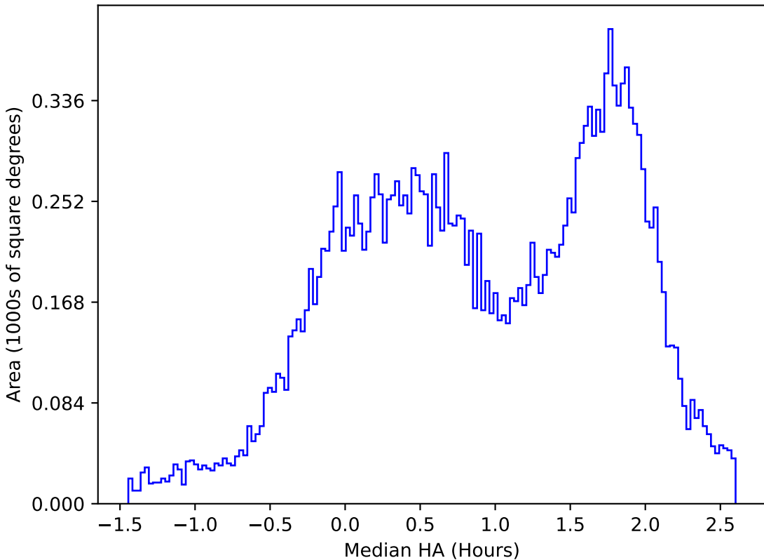
too_elab_r16_d3_gz_v3.4_10yrs All sky u band: Median HA
