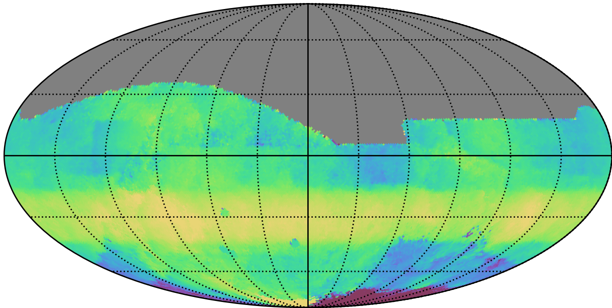
too_elab_r16_d3_gz_v3.4_10yrs All sky r band: Median HA
