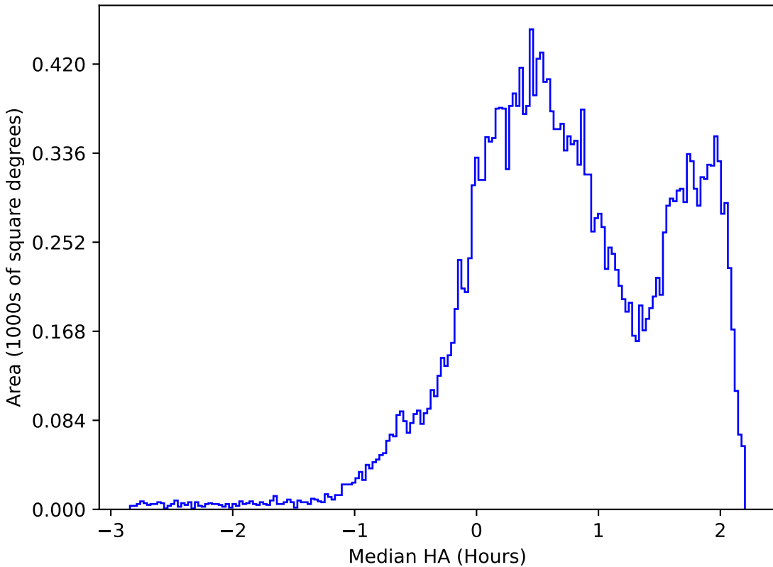
too_elab_r16_d3_gz_v3.4_10yrs All sky r band: Median HA
